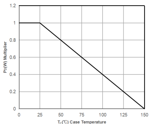
Figure 3. Power Dissipation
