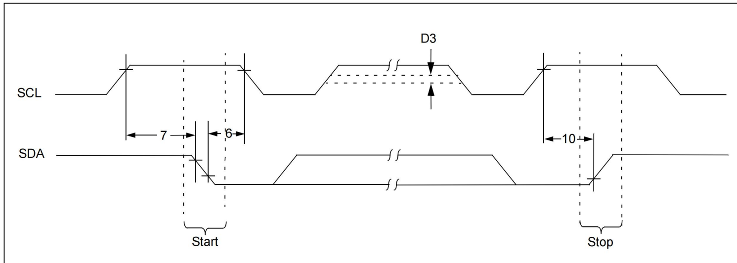
FIGURE 1-2: BUS TIMING START/STOP
