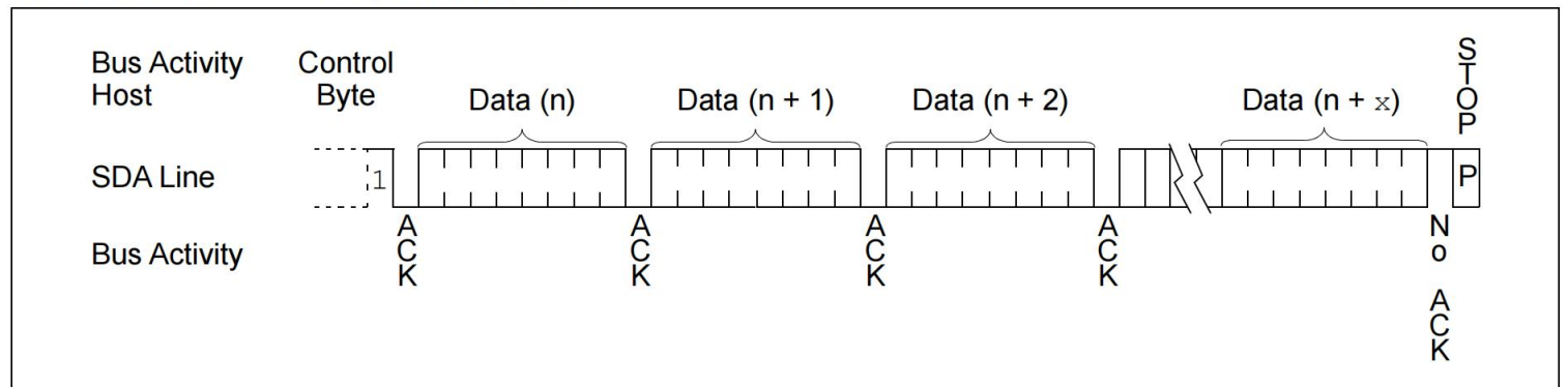
FIGURE 8-3: SEQUENTIAL READ
