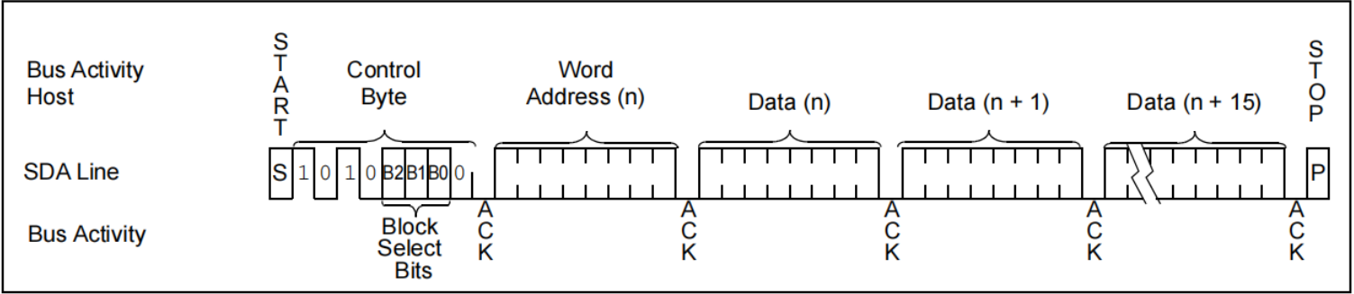
FIGURE 6-2: PAGE WRITE
