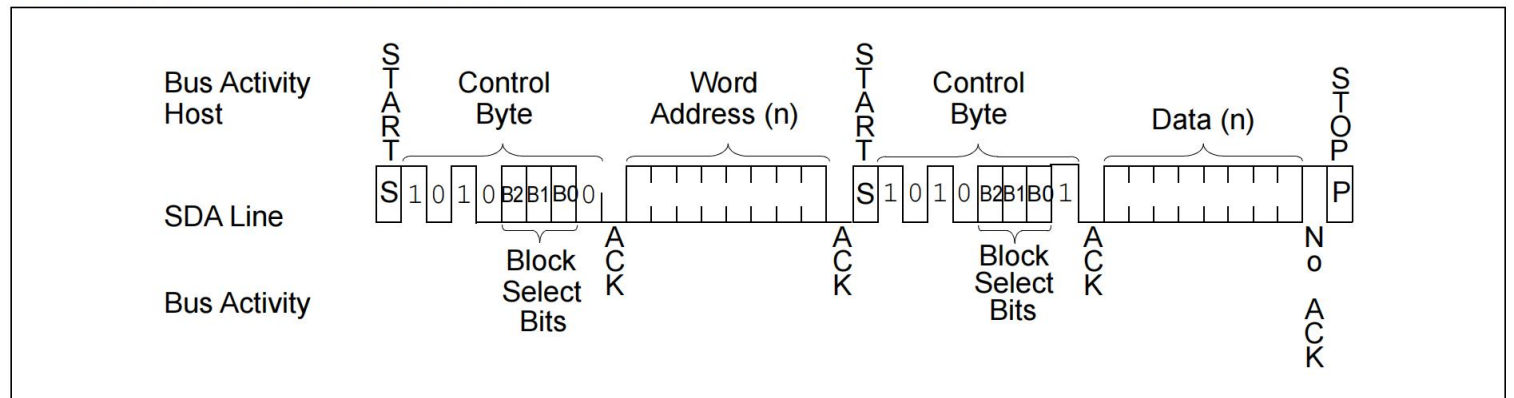
FIGURE 8-2: RANDOM READ
