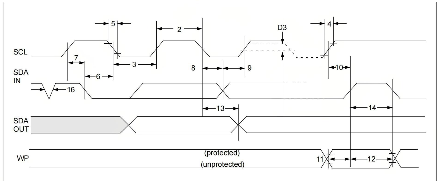
FIGURE 1-1: BUS TIMING DATA
