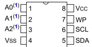
PDIP (Top View)
