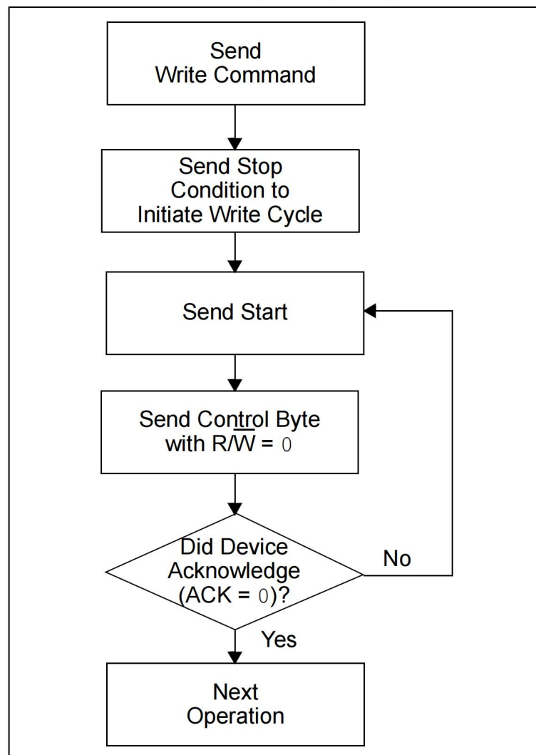
FIGURE 7-1: ACKNOWLEDGE POLLING FLOW
