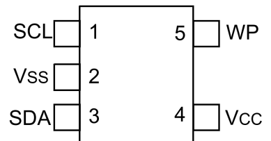
SOT-23 (Top View)
