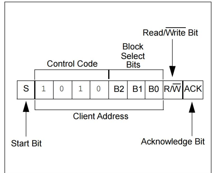
FIGURE 5-1: CONTROL BYTE ALLOCATION
