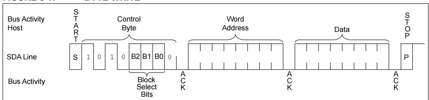
FIGURE 6-1: BYTE WRITE
