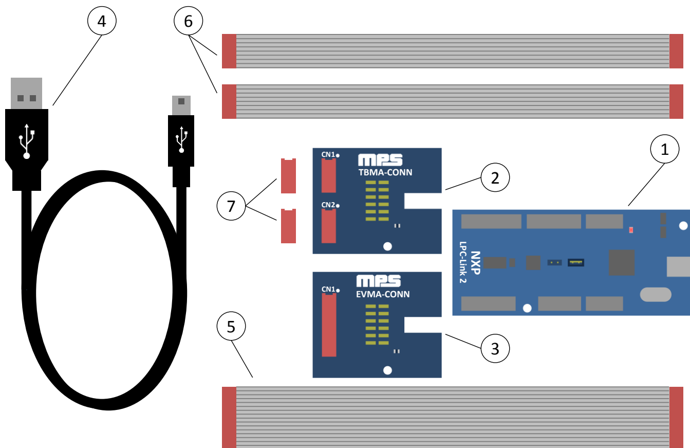
Figure 2: Kit Contents
