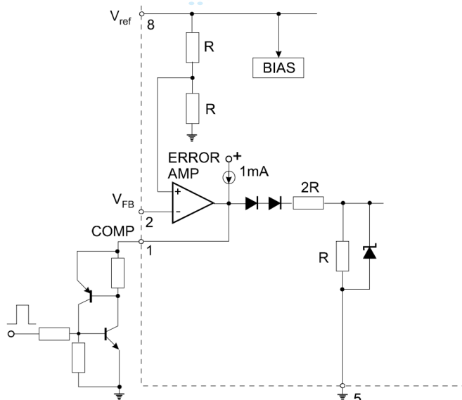
Figure 5. Latched Shutdown
