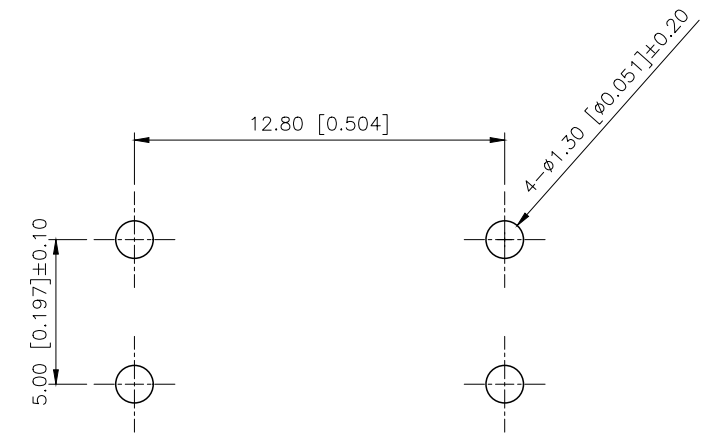
PCB LAYOUT
