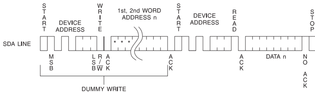
Figure 5. Random Read
