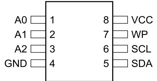
8-lead SOIC
