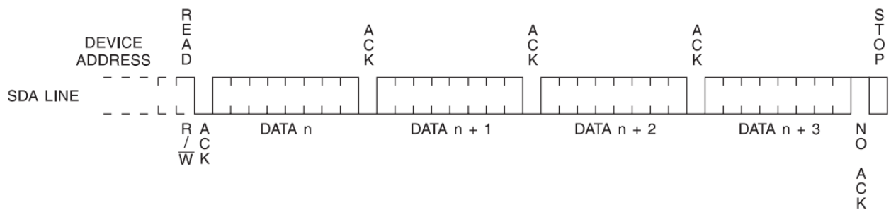
Figure 6. Sequential Read
