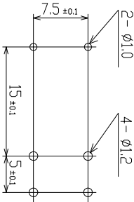
DRILLING DIAGRAM(BOTTOM VIEW)
