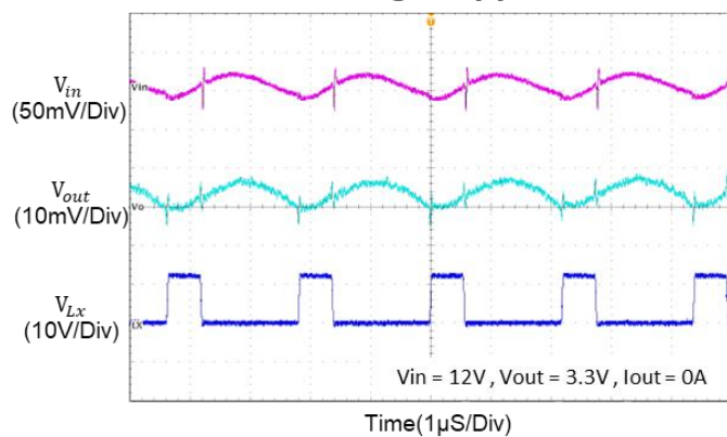
Voltage Ripple
