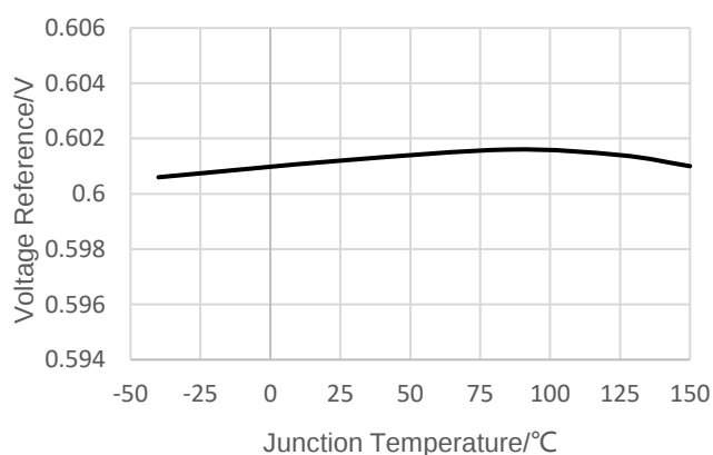
Voltage Reference vs Temperature
