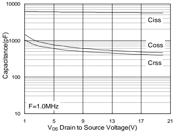
Fig.7 Capacitance
