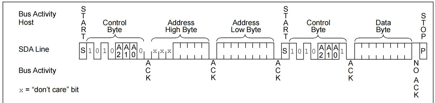
FIGURE 8-2: RANDOM READ
