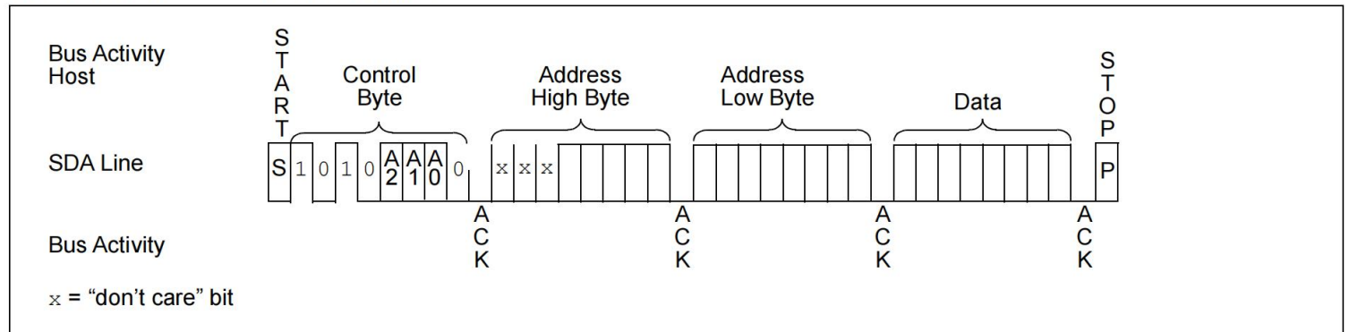
FIGURE 6-1: BYTE WRITE
