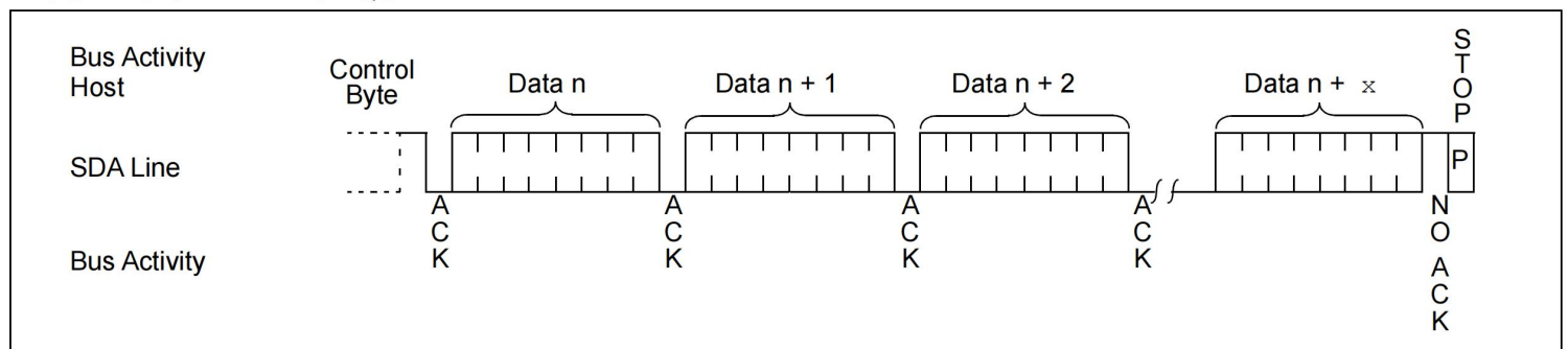
FIGURE 8-3: SEQUENTIAL READ
