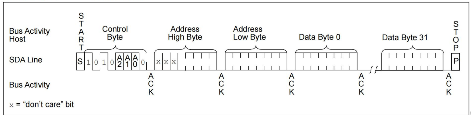
FIGURE 6-2: PAGE WRITE
