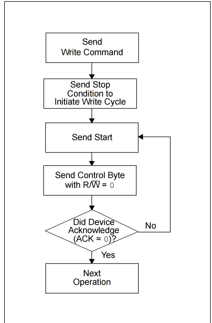
FIGURE 7-1: ACKNOWLEDGE POLLING FLOW
