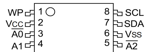
X-Rotated TSSOP (X/ST)
