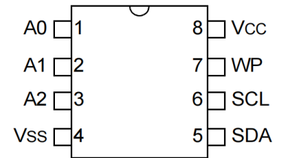
PDIP/SOIC
