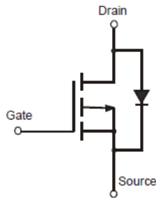
Equivalent Circuit
