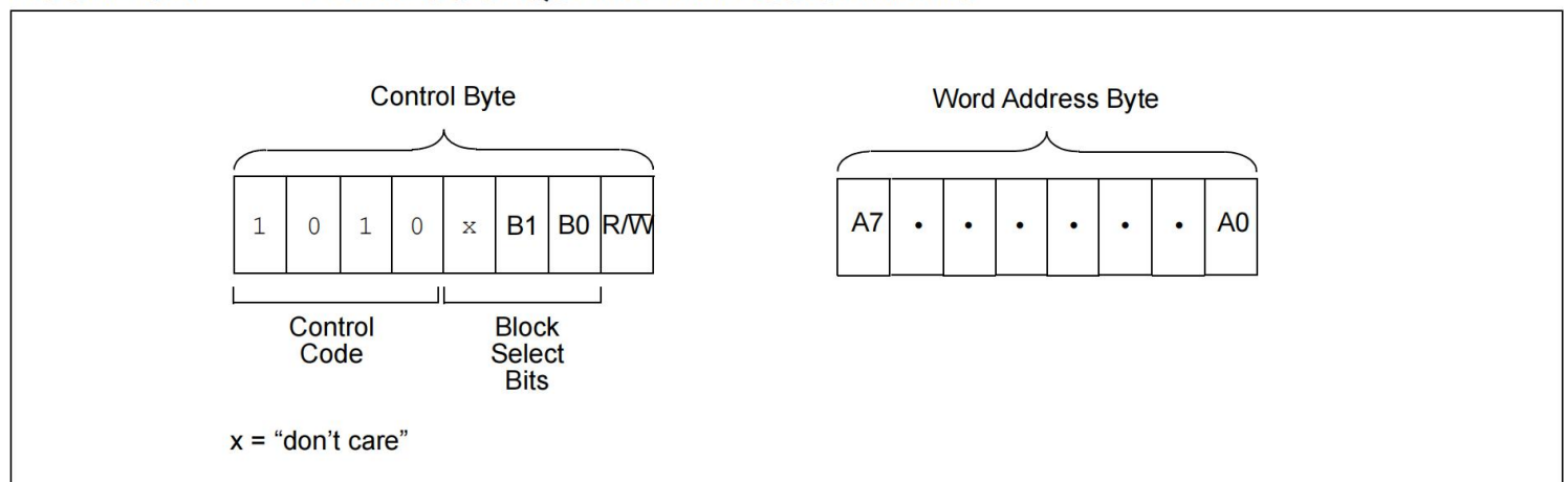
FIGURE 5-2: ADDRESS SEQUENCE BIT ASSIGNMENTS
