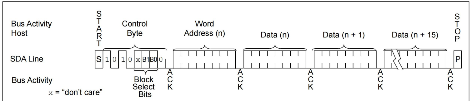
FIGURE 6-2: PAGE WRITE
