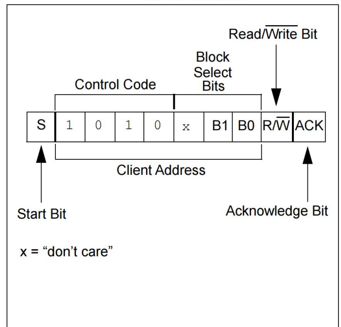
FIGURE 5-1: CONTROL BYTE ALLOCATION
