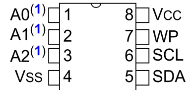
PDIP/MSOP (Top view)
