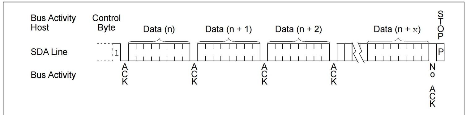
FIGURE 8-3: SEQUENTIAL READ
