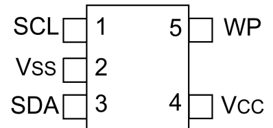
SOT-23 (Top view)
