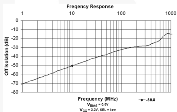
Figure 7. Off Isolation
