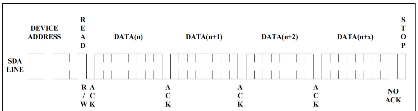
Figure 10. Sequential Read
