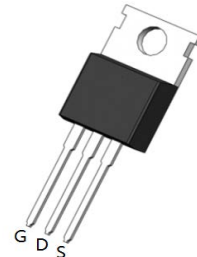
TO-220
