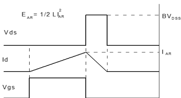
Figure 3: Unclamped Inductive Switching Test Circuit & Waveform
