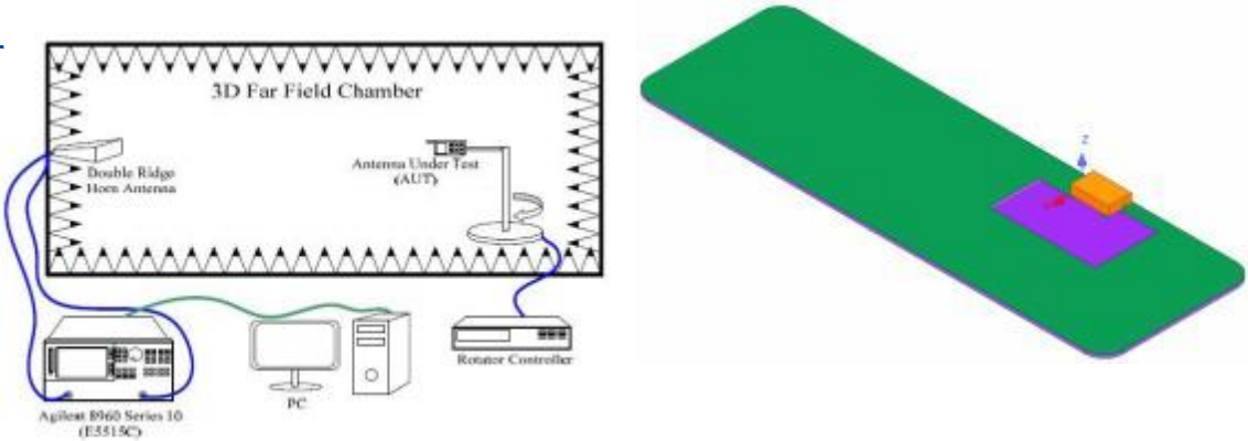
Fig.2 FAR-field Chamber
