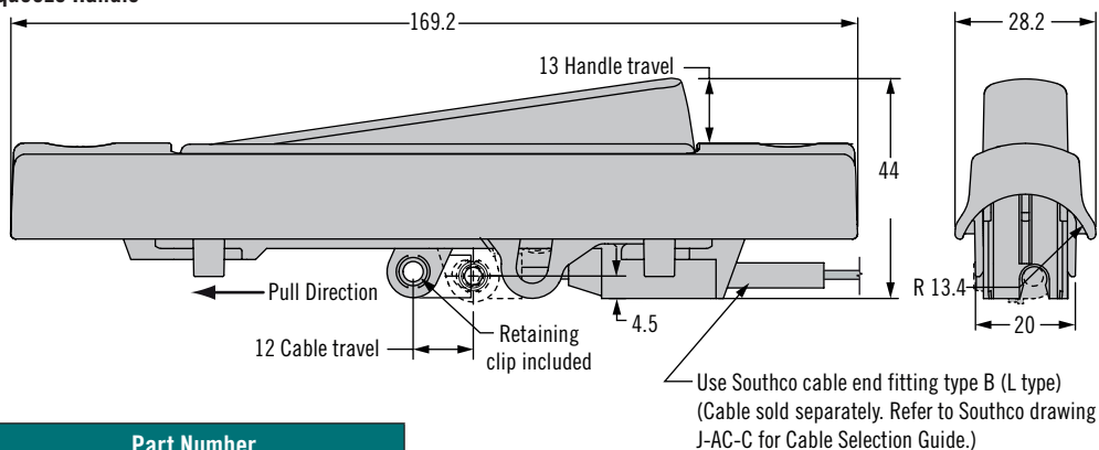
Squeeze Handle
