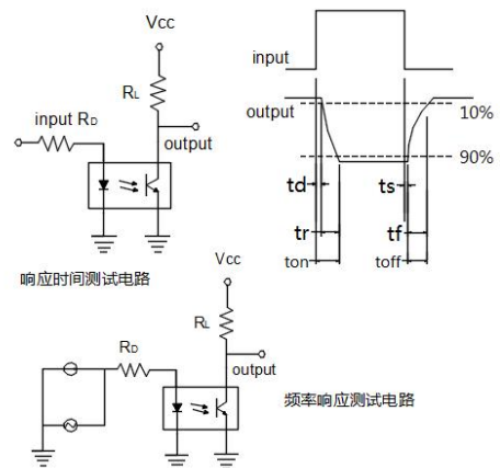
Fig.10 Switching Time Test Circuit & Waveforms
