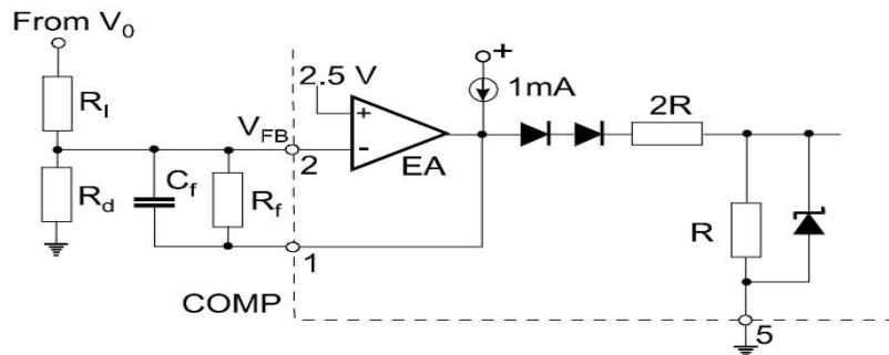
Figure 5. Latched Shutdown
