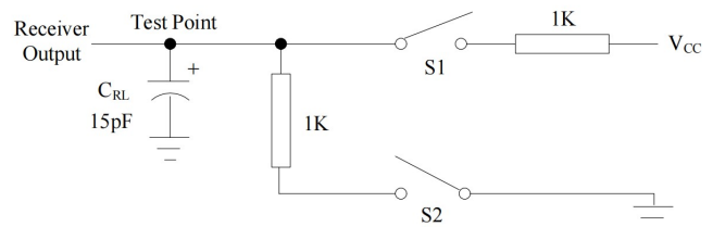
Figure 5. Receiver Enable/Disable Timing Test Load
