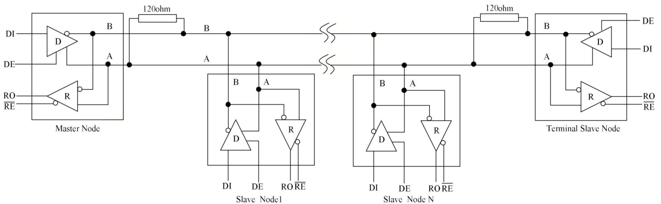
Figure 1. Typical Half-Duplex RS-485 Network
