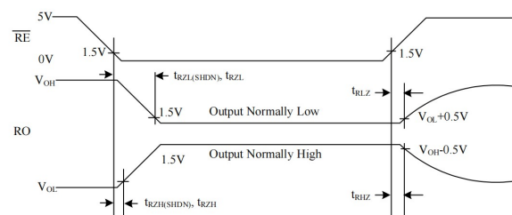
Figure 10. Receiver Enable and Disable Times
