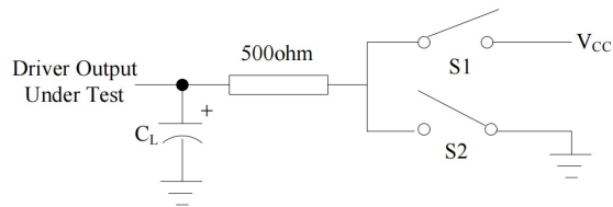
Figure 4. Driver Enable/Disable Timing Test Load
