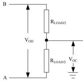
Figure 2. Driver DC Test Load
