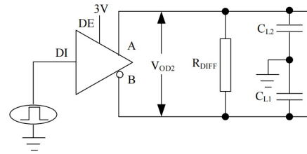
Figure 3. Driver Timing Test Circuit
