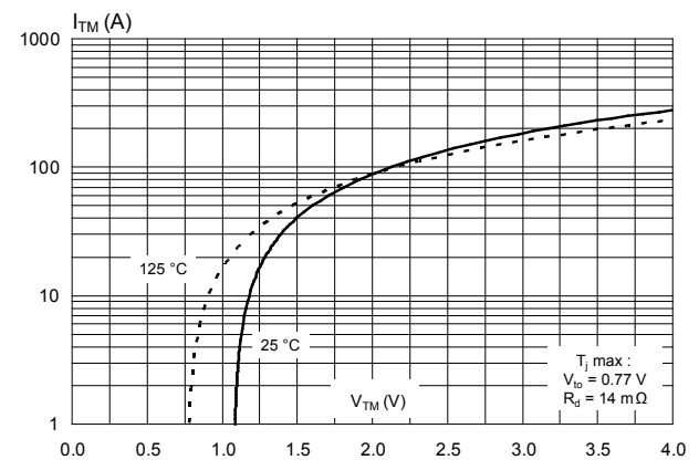
Figure 8. On-state characteristics (maximum values)
