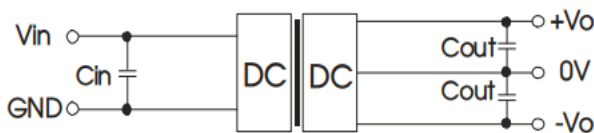
Figure 1: Application circuit
