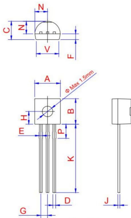
TO-92
