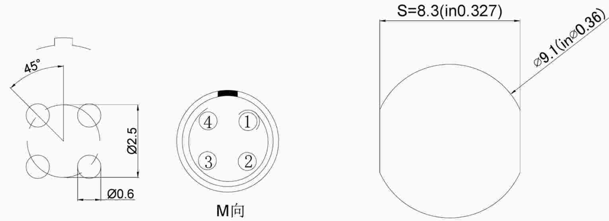
Pcb plate opening size (PCB板开孔尺寸)
