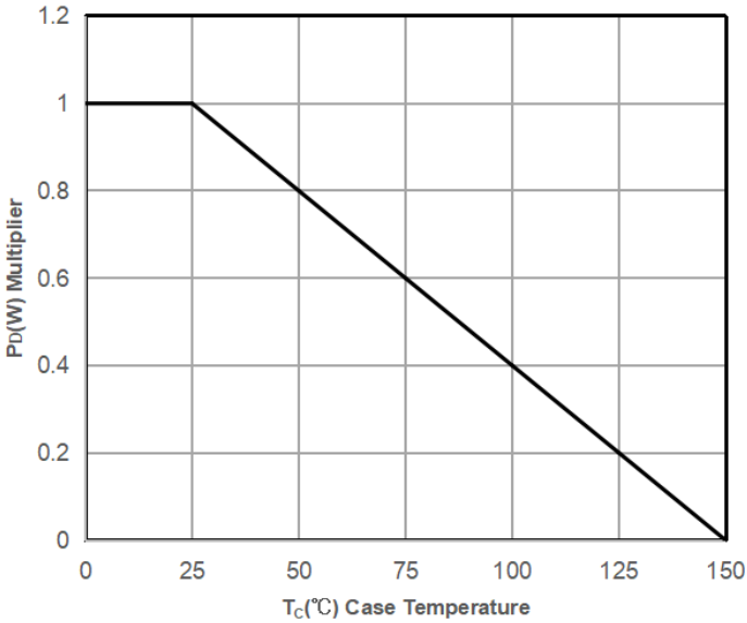
Power Capability
