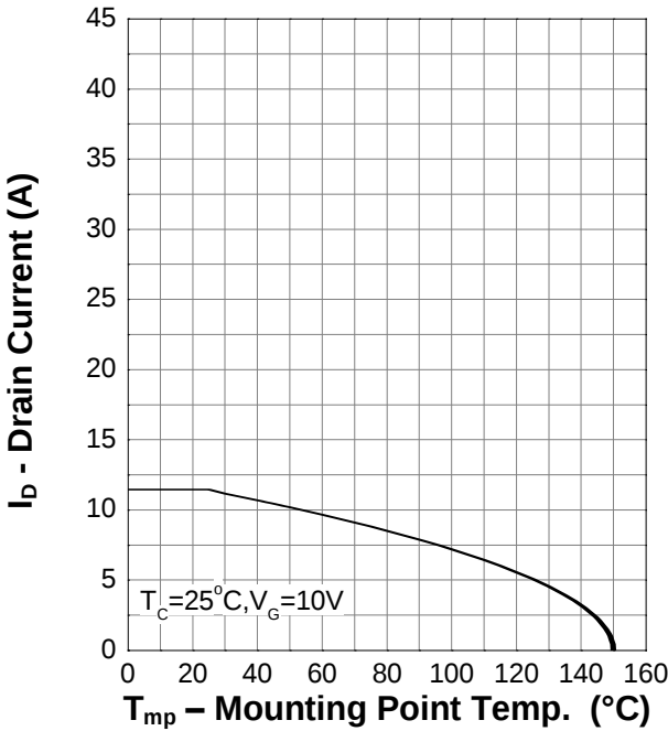
Current Capability
