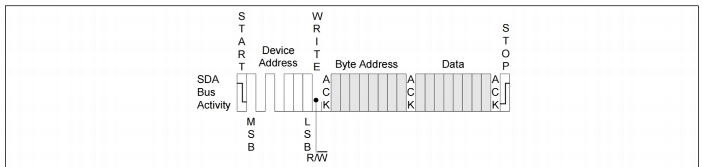
Figure . Byte Write
