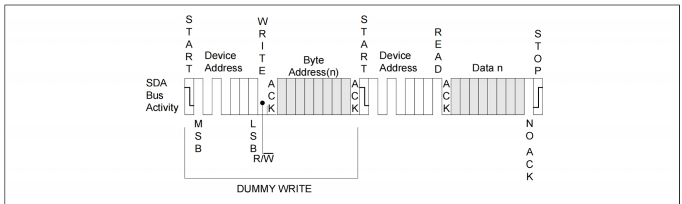
Figure . Random Address Read
