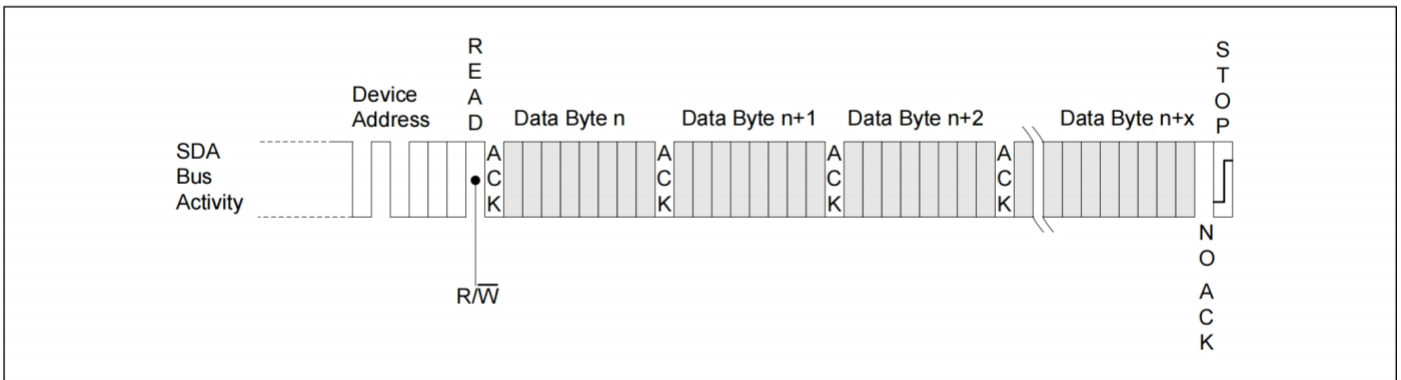
Figure . Sequential Read
