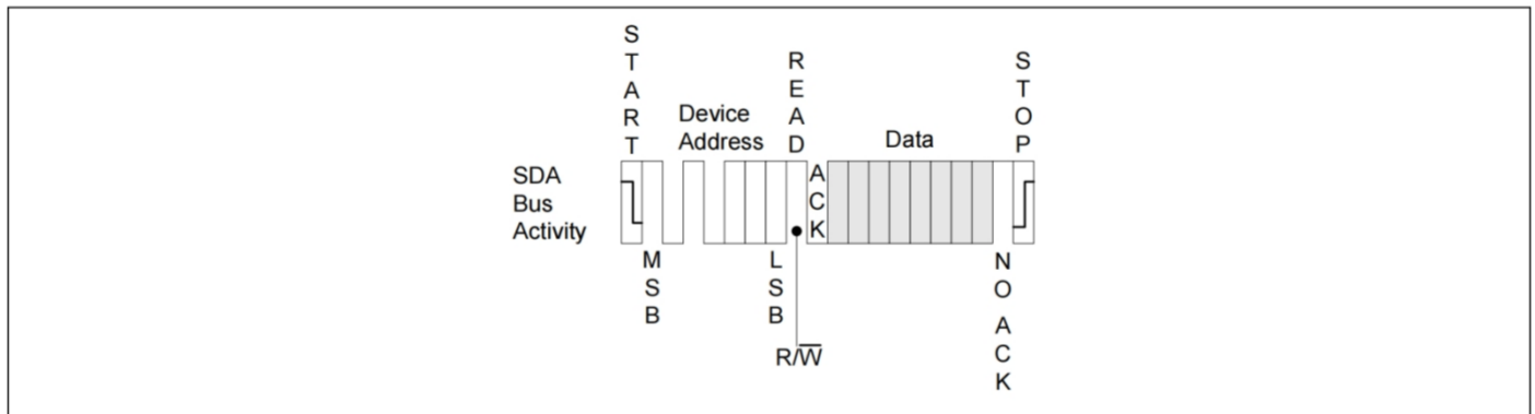
Figure . Current Address Read
