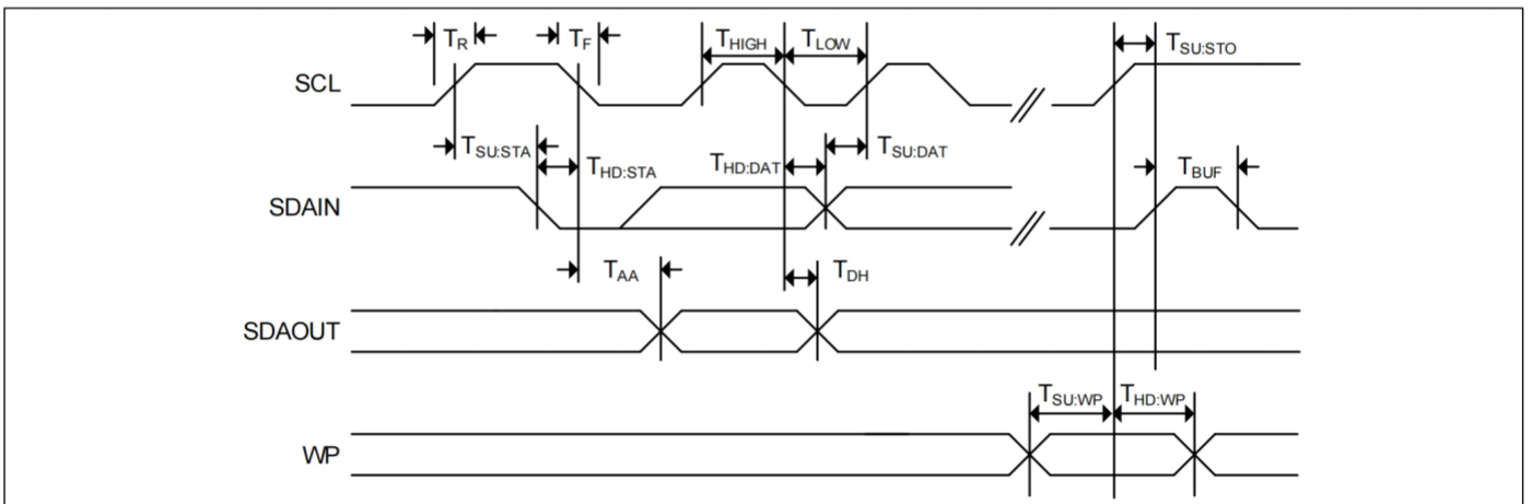
Figure . Write Cycle Timing
