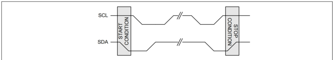
Figure . Start and Stop Conditions
