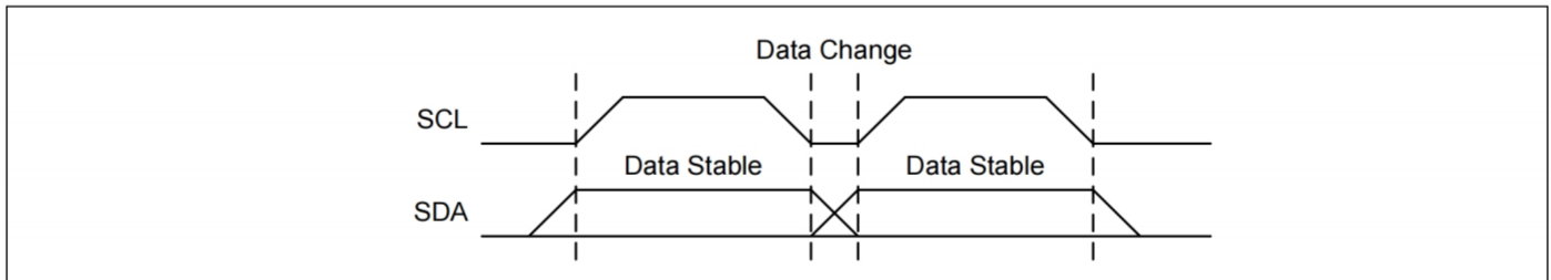
Figure . Data Validity Protocol
