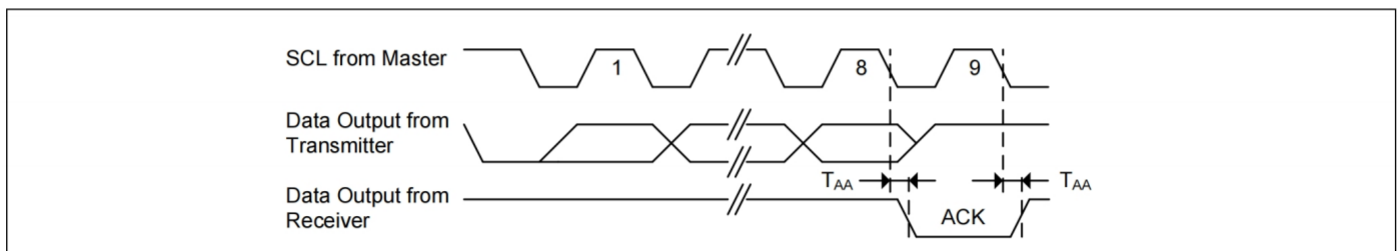
Figure . Output Acknowledge
