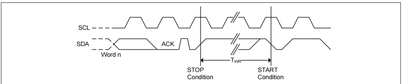
Figure . Write Cycle Timing
