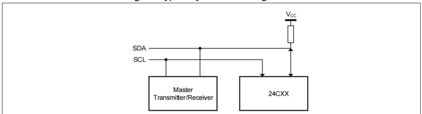
Figure . Typical System Bus Configuration
