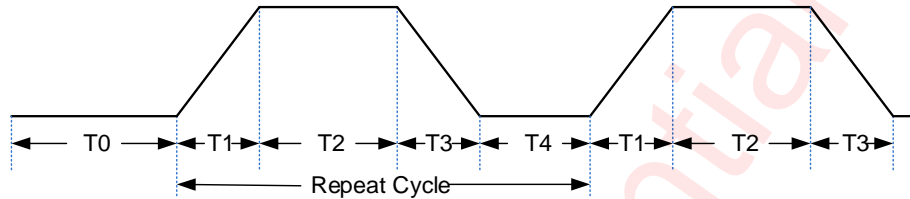
Figure 10 LED Breath Timing in Pattern Mode
