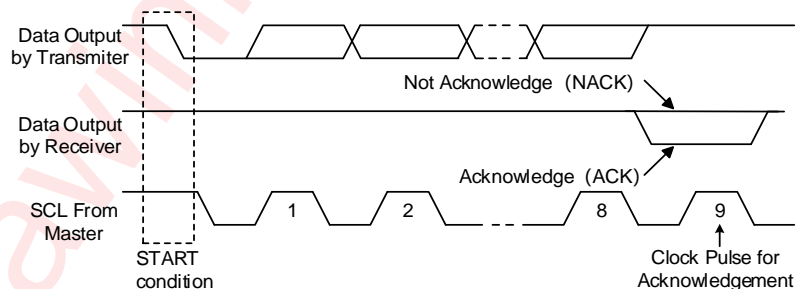
Figure 7 I 2 C ACK Timing
