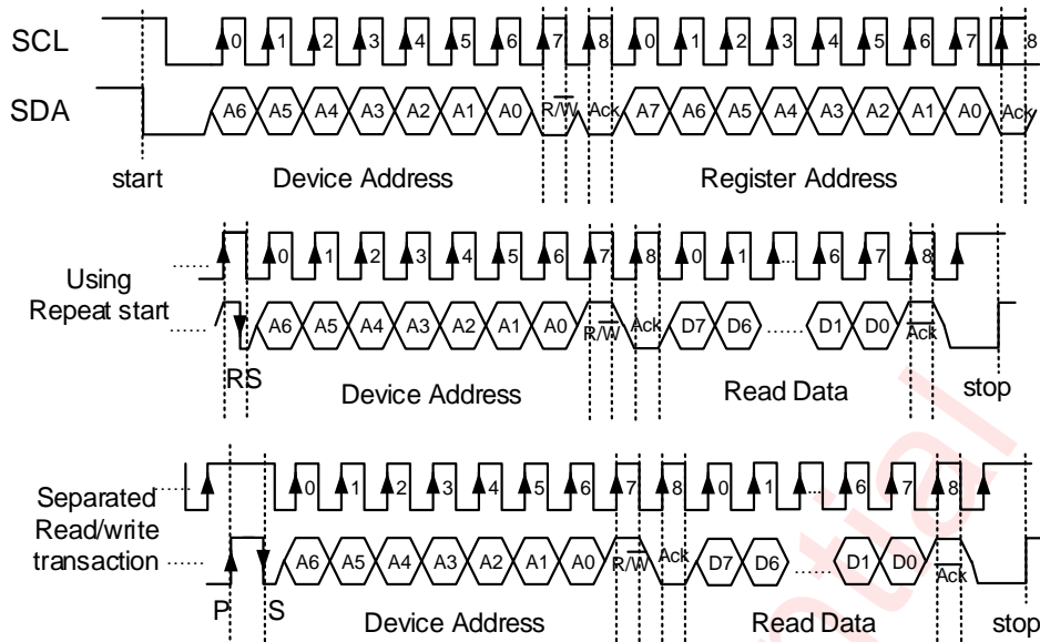
Figure 9 I 2 C Read Byte Cycle
