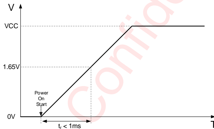
Figure 3 AW2023 Power on Timing
