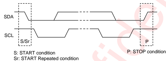
Figure 6 I 2 C Start/Stop Condition Timing
