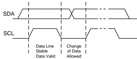
Figure 5 Data Validation Diagram
