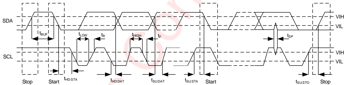
Figure 2 Timing of I 2 C Interface Signals
