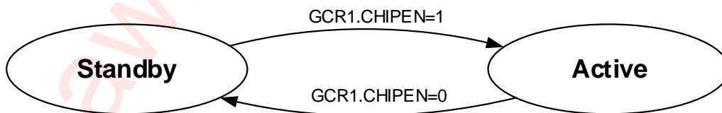
Figure 4 AW2023 Operating Modes Transition
