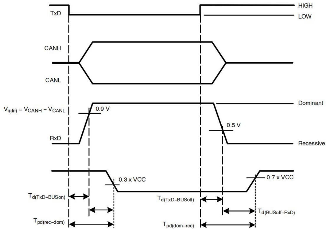
Figure 8. Timing Diagram for AC Characteristics
