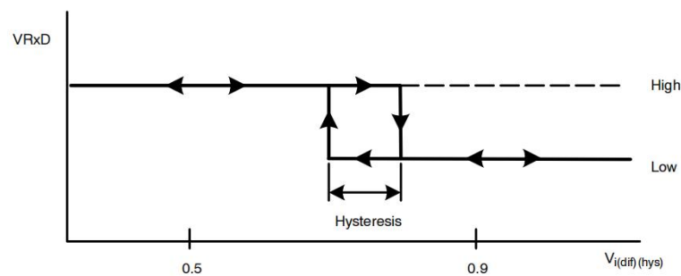
Figure 6. Hysteresis of the Receiver
