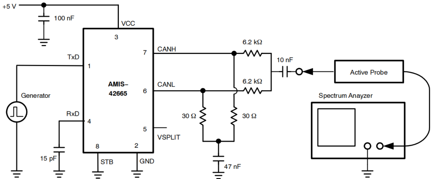
Figure 11. Basic Test Setup for Electromagnetic Measurement
