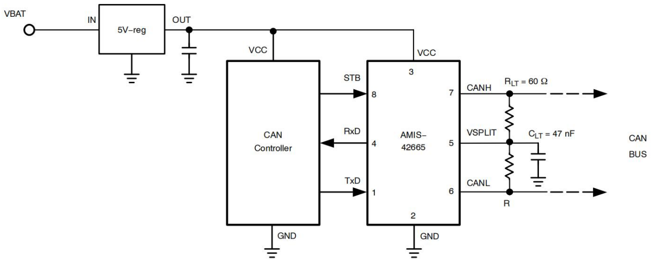
Figure 2. Application Diagram
