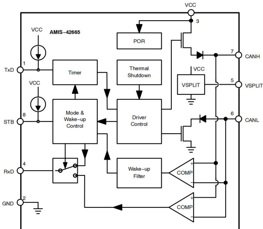
Figure 1. Block Diagram
