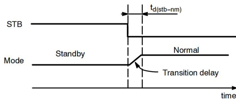
Figure 9. Transition from Standby to Normal
