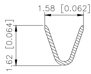
SECTION:A-A SCALE:1:1
