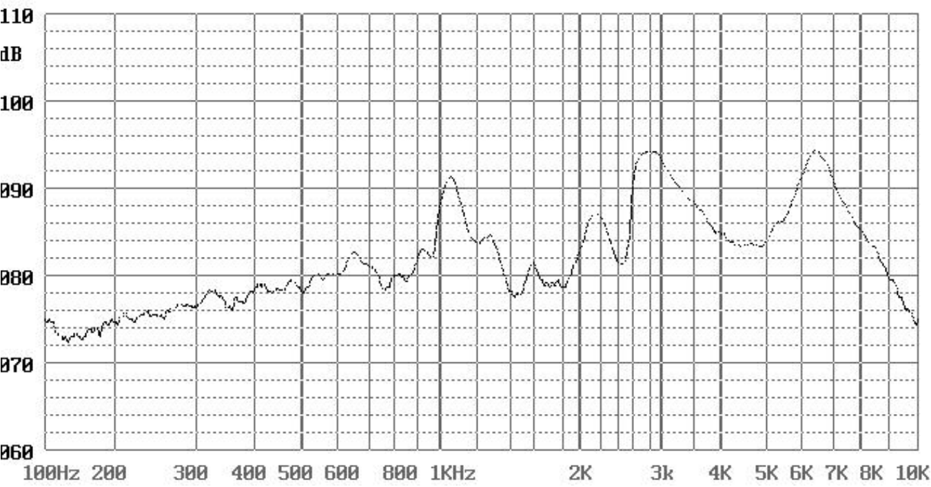
Typical Frequency Response Curve（音频曲线图）
