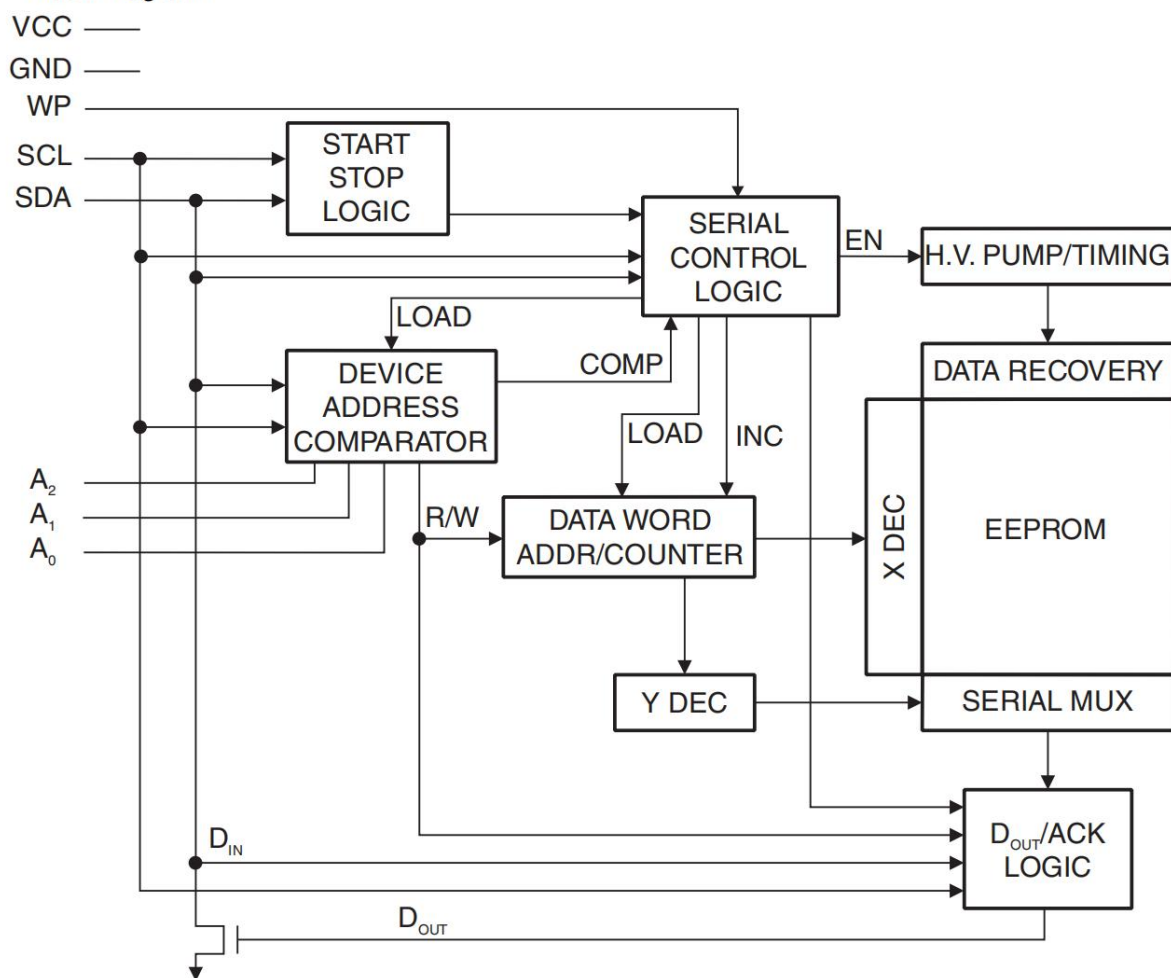
Figure 0-1. Block Diagram
