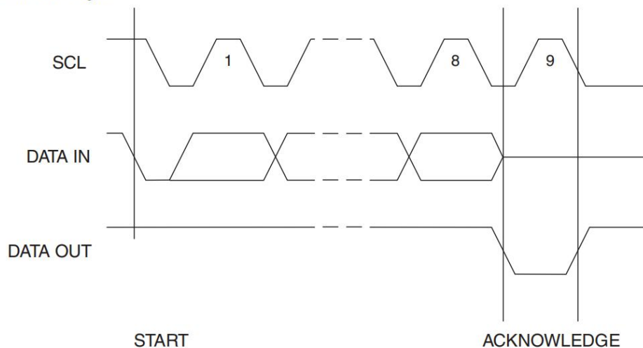
Figure 3-6. Output Acknowledge
