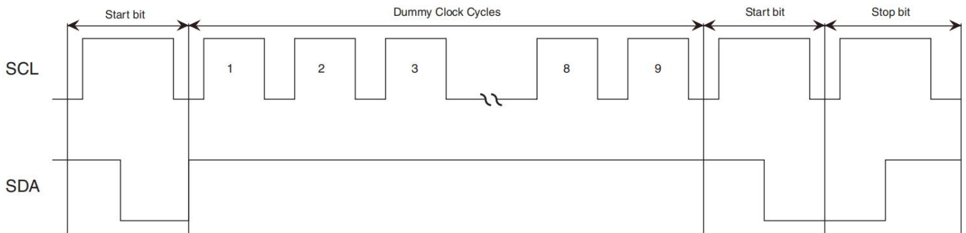
Figure 3-1. Protocol Reset Condition
