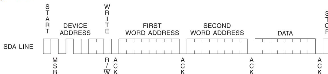
Figure 6-2. Byte Write
