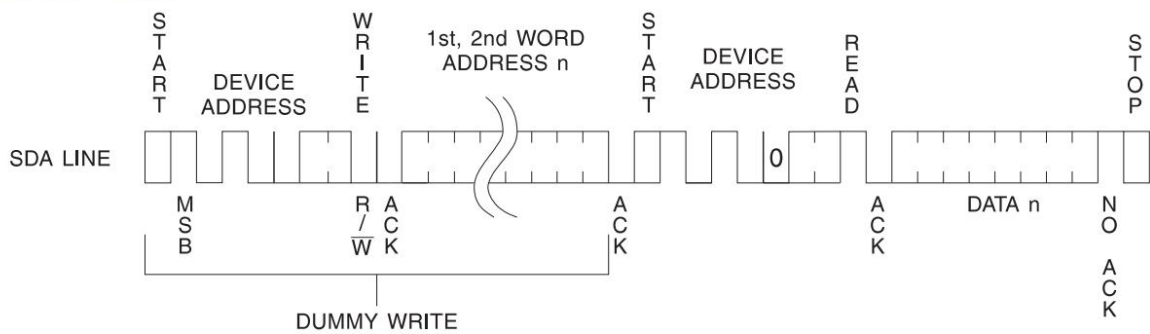
Figure 6-5. Random Read
