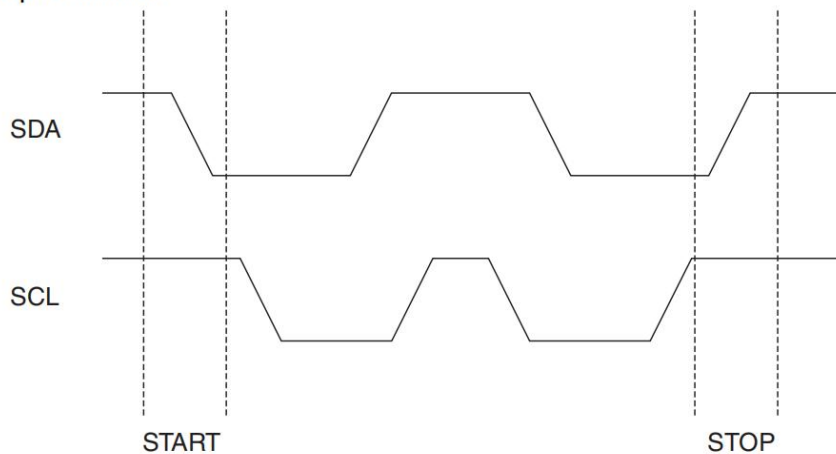
Figure 3-5. Start and Stop Definition
