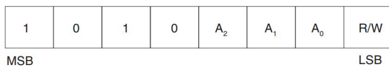
Figure 6-1. Device Address
