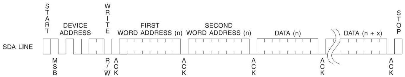
Figure 6-3. Page Write
