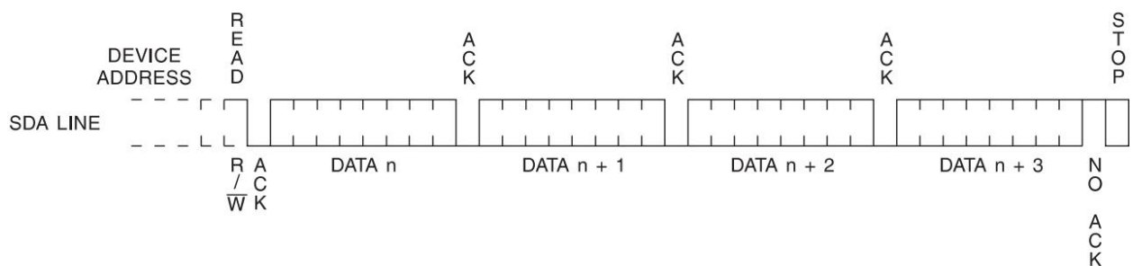
Figure 6-6. Sequential Read
