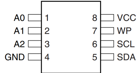
8-lead SOIC
