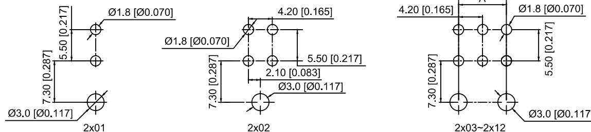
PCB LAYOUT :Component Side Recommended PCB Thickness 1.78MAX
