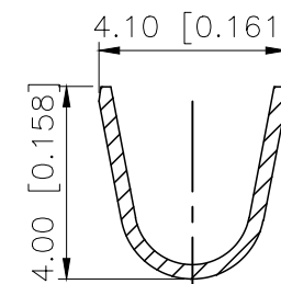
SECTION:B-B SCALE:1:1
