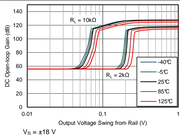
Figure 24. Open-Loop Gain vs Output Voltage Swing to Supply
