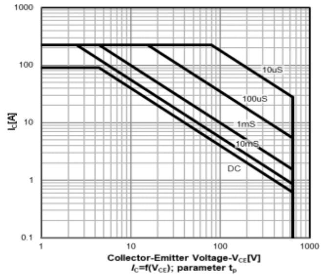
Safe operating area T_a=25\text{ }^\circ\text{C}
