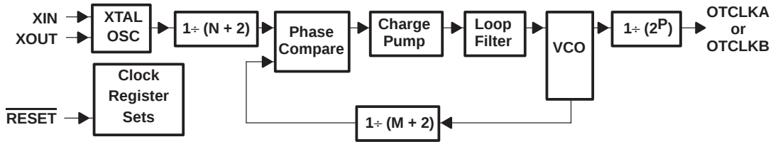
Figure 2–4. Clock Synthesizer Block Diagram
