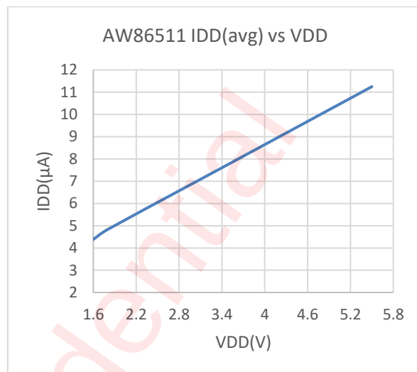
Average Supply Current vs. Supply Voltage T_a=25^{\circ}C
