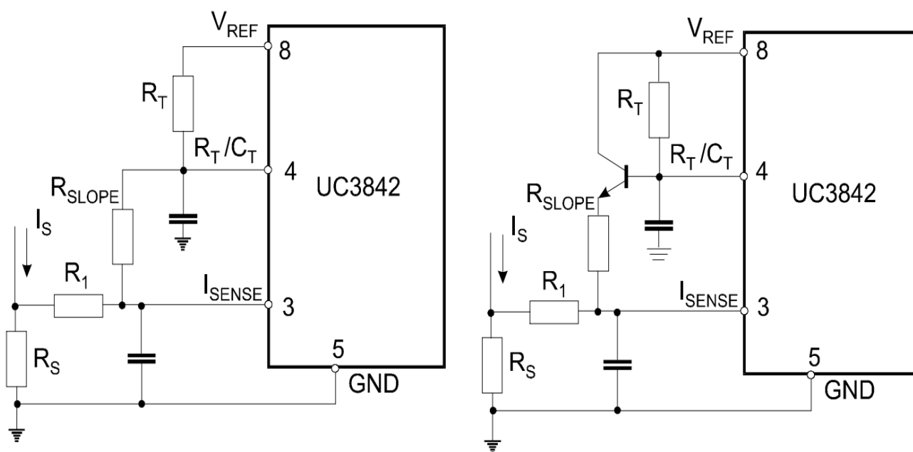
Figure 4. Slope Compensation Techniques
