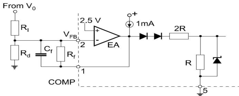
Figure 5. Latched Shutdown
