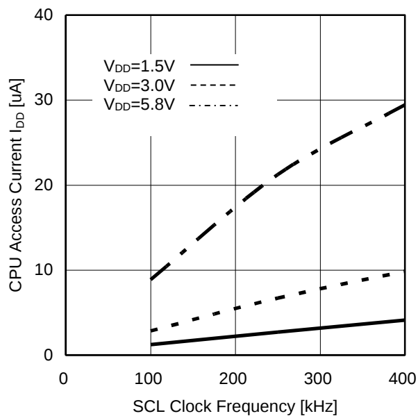
Figure 10. CPU Access Current vs. SCL Clock Frequency (with no 32-kHz clock output, SDA="H") (other pins open, C_{GOUT}=C_{DOUT}=0pF , T_{opt}=25^{\circ}C )
