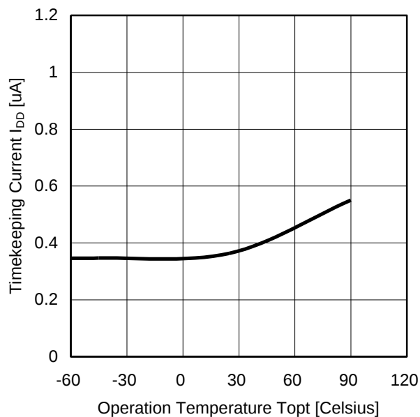
Figure 8. Timekeeping Current vs. Operating Temperature (with no 32-kHz clock output, output pins open) ( C_{GOUT}=C_{DOUT}=0pF , V_{DD}=3V )
