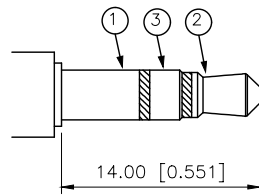
ø3.50 MATE PLUG
