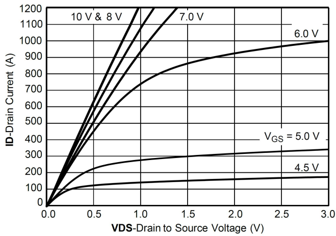
Output Characteristics
