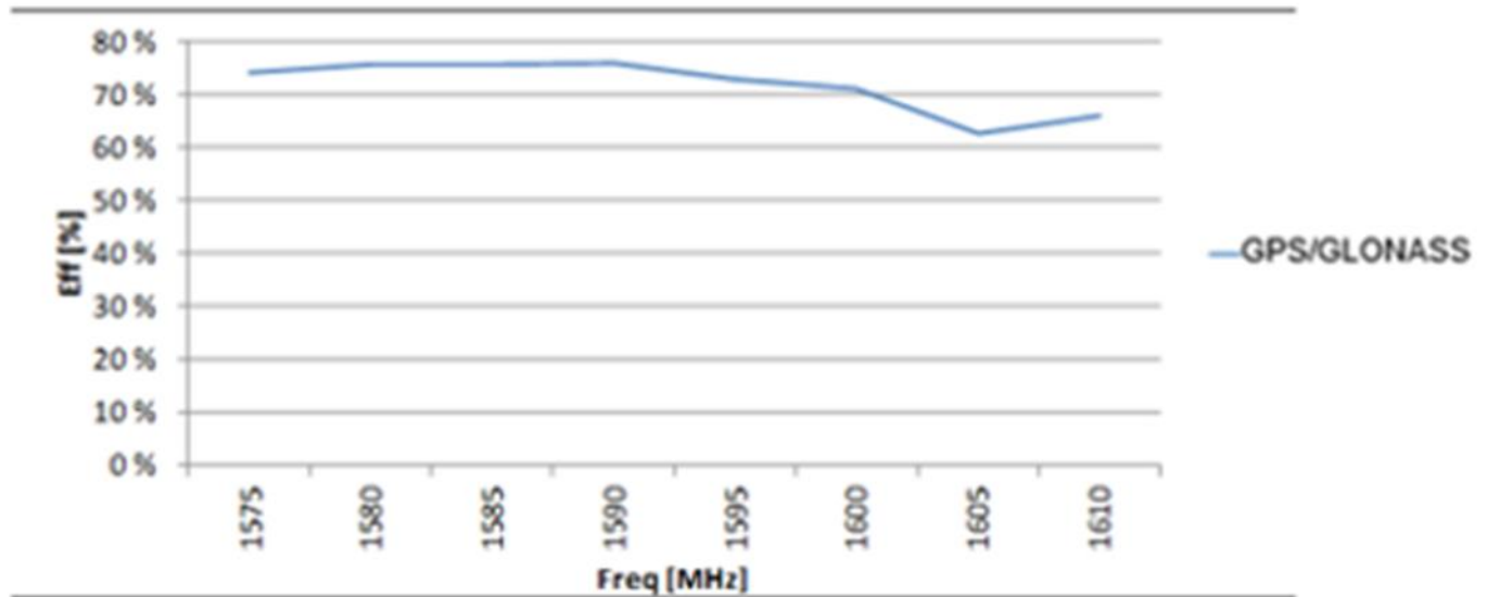
Typical Antenna Total Efficiency
