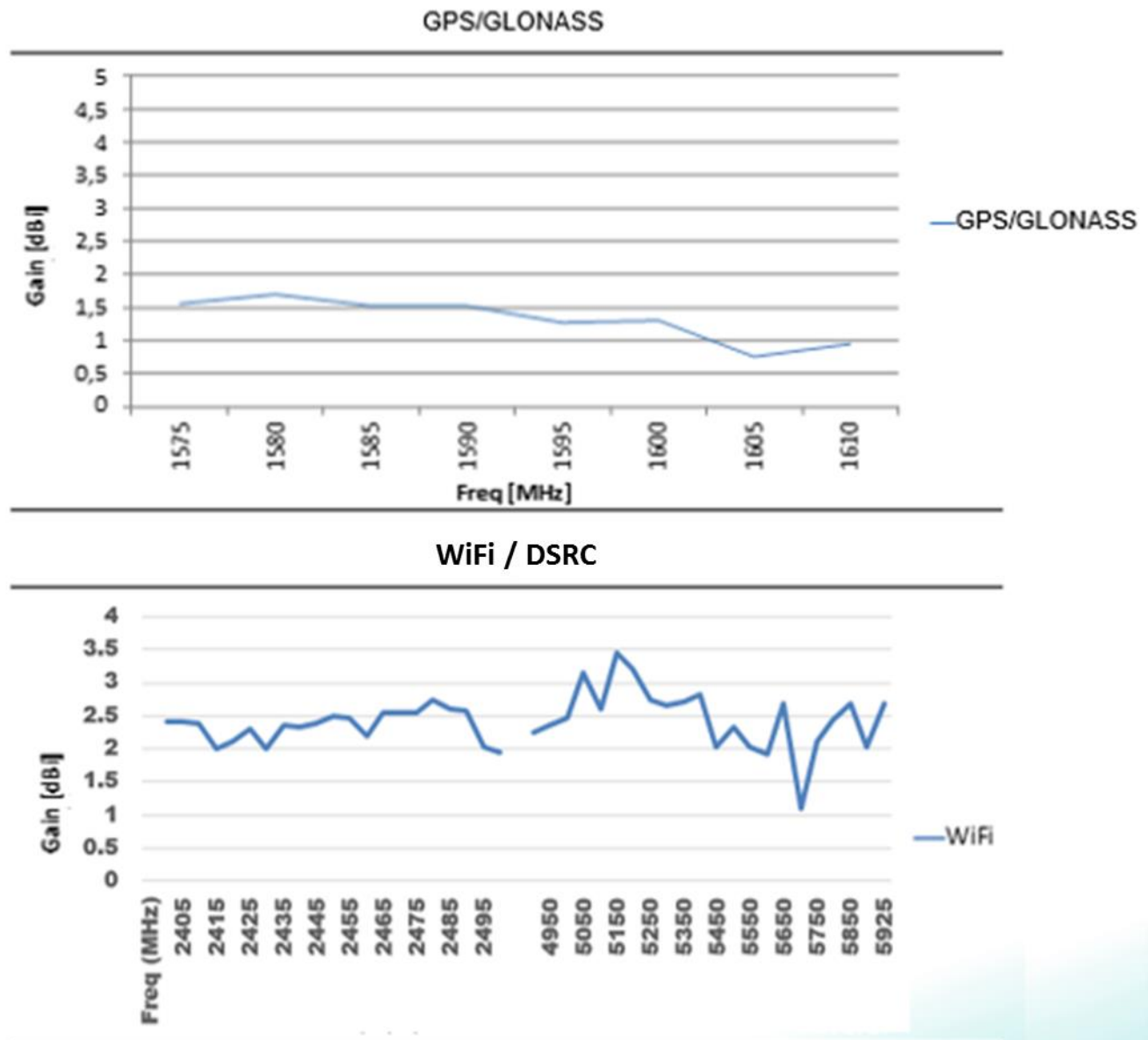
Typical Antenna Peak Gain
