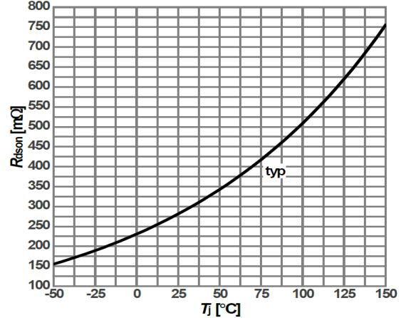
Figure 12: On-Resistance vs Temperature
