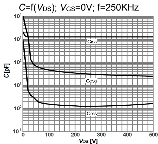
Figure 16: Typ. capacitances
