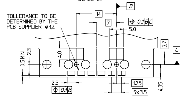
PCB LAYOUT (COMPONENT SIDE) SCALE 2:1
