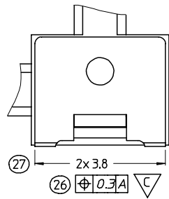
DETAIL1 SCALE 10:1
