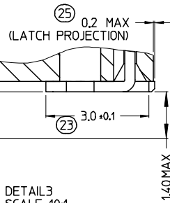
DETAIL3 SCALE 10:1
