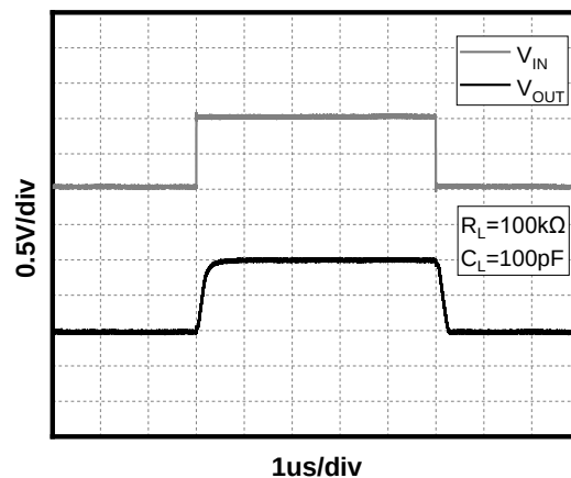
Figure 9. Large-Signal Step Response( V_S=1.5\text{V} )
