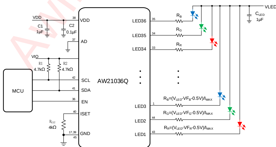
Figure 1 AW21036Q Application Circuit
