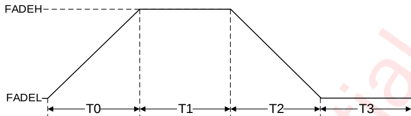
Figure 16 LED Breath Timing in Pattern Mode
