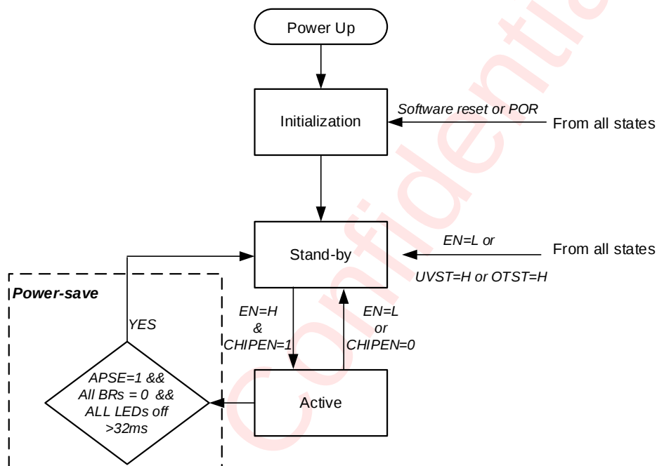
Figure 8 AW21036Q Operating Mode Transition
