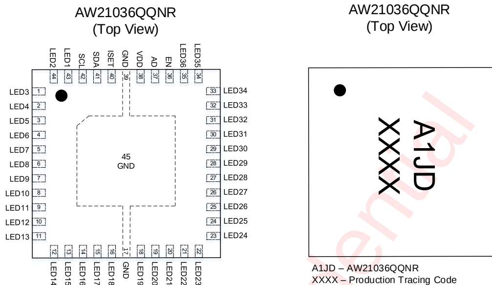
Figure 2 Pin Configuration and Marking
