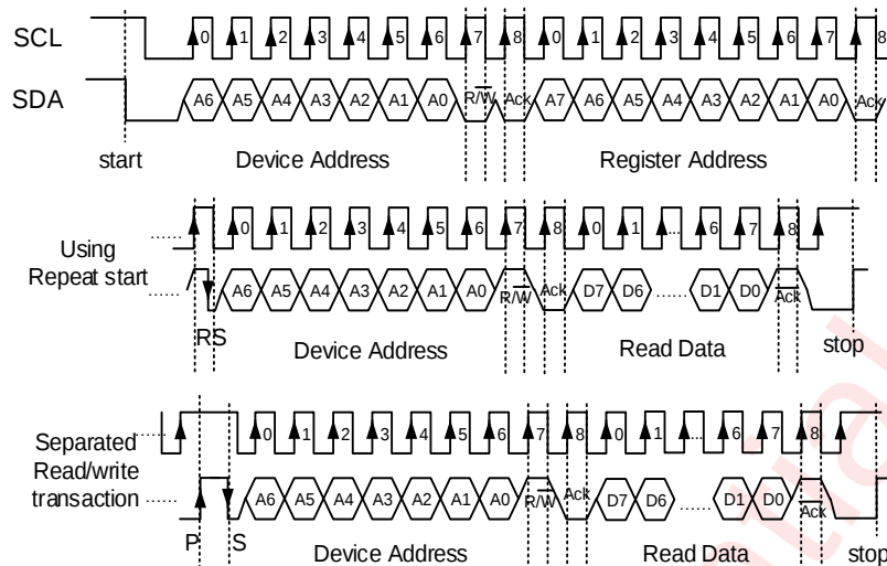
Figure 13 I²C Read Byte Cycle
