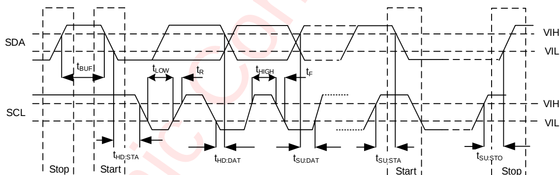
Figure 5 I 2 C Interface Timing
