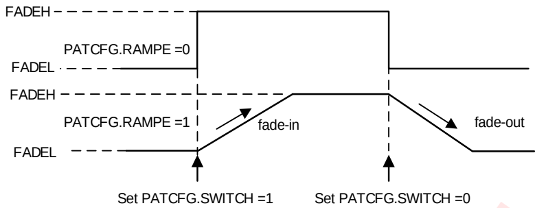
Figure 17 Manual Control Mode
