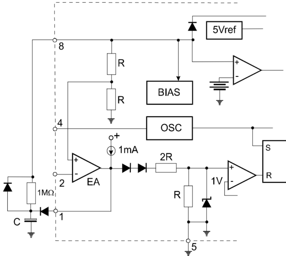
Figure 8. Soft-Start Circuit
