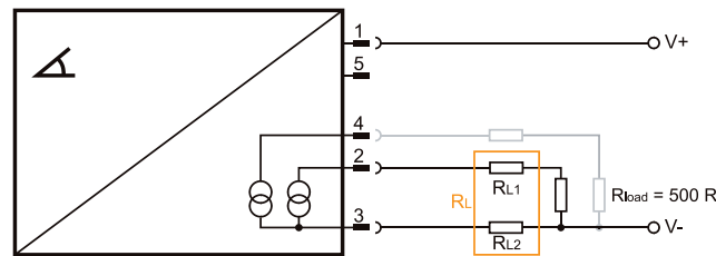
Figure 20: Length of cable for current output
