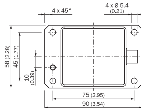
Figure 17: Dimensional drawing TMx88 (aluminum housing)
